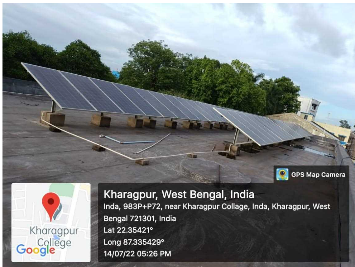
A 20 KW grid connected roof top solar photovoltaic plant is installed with the financial support of Government of west Bengal under Aloshree Prakalpa
